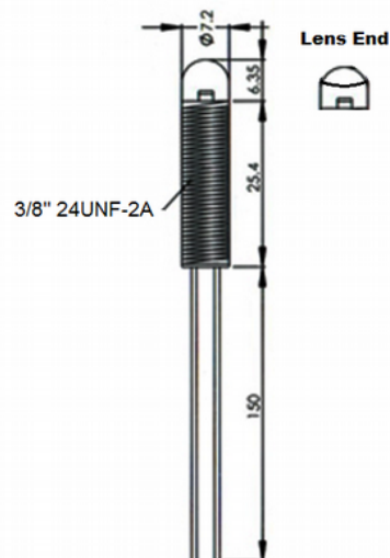
Precision-Focused Lens End & Half-Spherical UNF 3/8 " Wire
