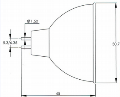
Precision-Focused Lens End & Half-Spherical UNF 1/2" Bi Pin
