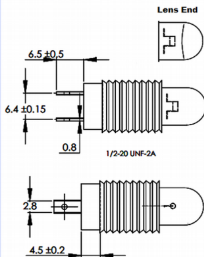
Precision-Focused Lens End & Half-Spherical UNF 1/2" Bi Pin
