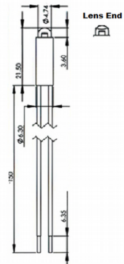
Precision-Focused Lens End & Half-Spherical Wire Lead
