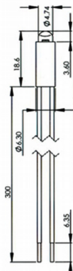
Precision-Focused Lens End (Short Base) Wire Lead
